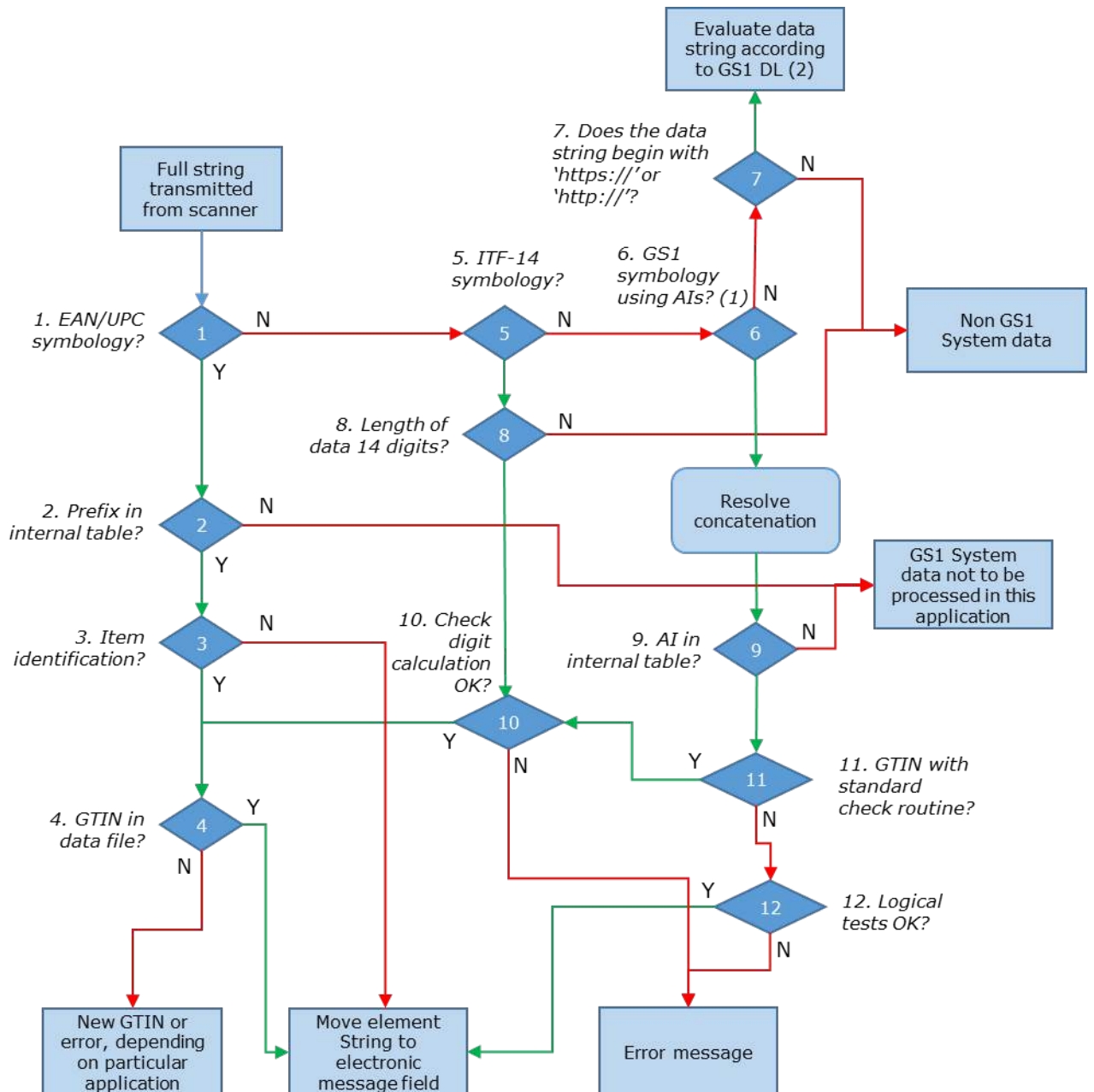
Figure 7.2.1-1. Test procedure
