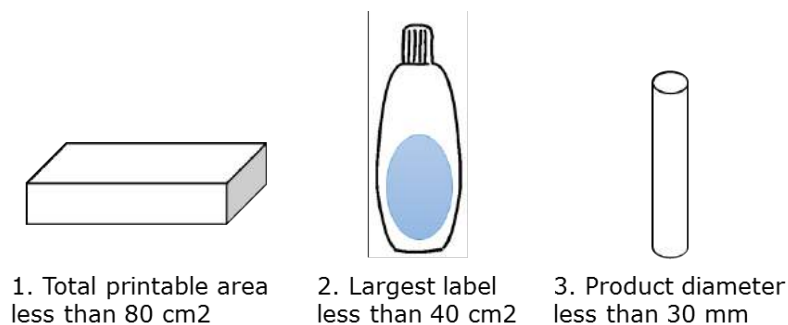
Figure 4.3.7-1. GTIN-8 packaging size constraints
