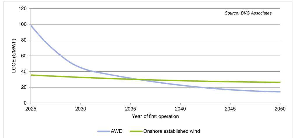
Figure 3: Trend in average Levelized Cost of Energy (LCOE) of AWE and onshore wind turbine technology.
